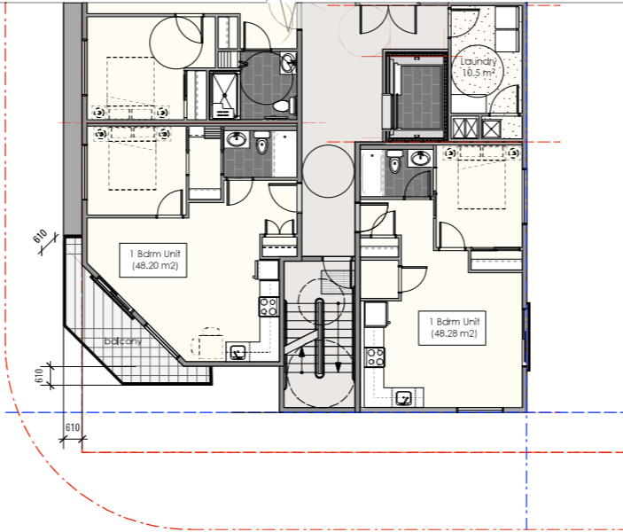
3RD FLOOR PLANS SCALE 1:100
