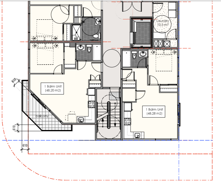
4TH FLOOR PLANS SCALE 1:100
