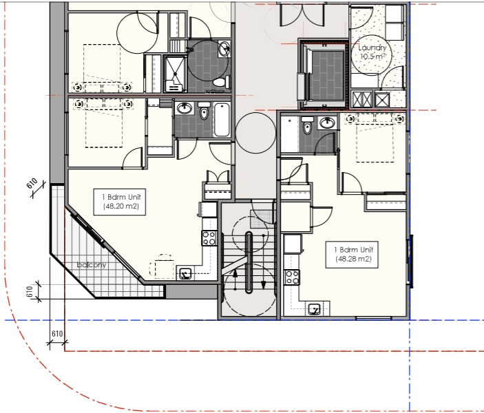
2ND FLOOR PLANS SCALE 1:100
