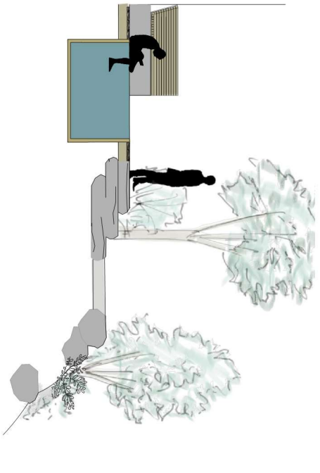
3 SOUTH PATIO SECTION L4.1 / 1:30
