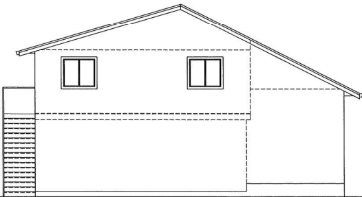
2 REAR ELEVATION 1/4"=1'-0"
