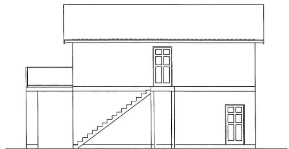
3 RIGHT ELEVATION 1/4"=1'-0"
