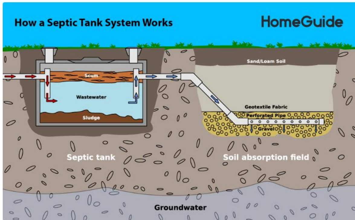
Figure 1. Example of a type one septic system (3).
